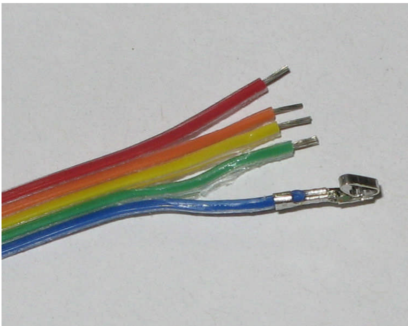
Figure 4: One Crimped
