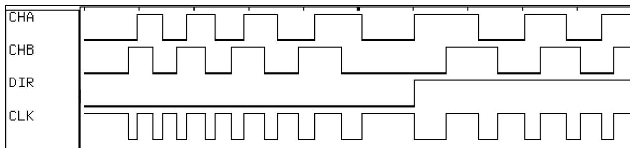
Figure 8: WW-12 Timing
