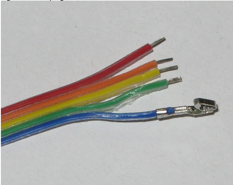
Figure 3: One Crimped
