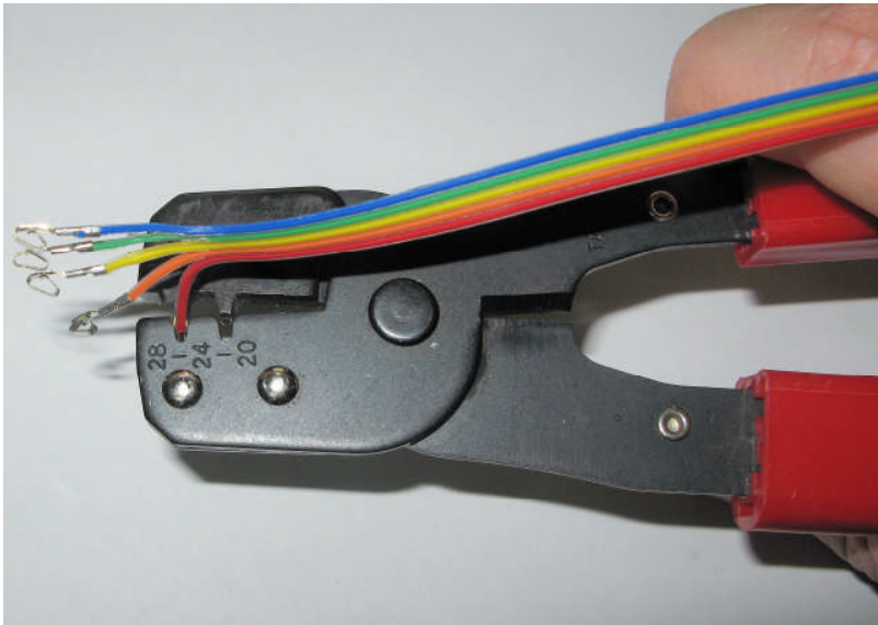
Figure 2: Crimping
